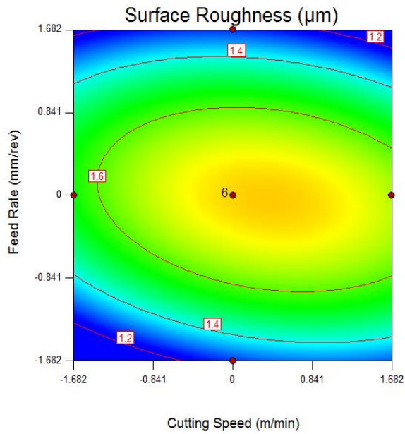
Fig5: Contour plot of surface roughness-Cutting speed and Feed rate
