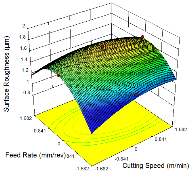
Fig6: Surface plot of Surface roughness-Cutting speed and Feed rate
