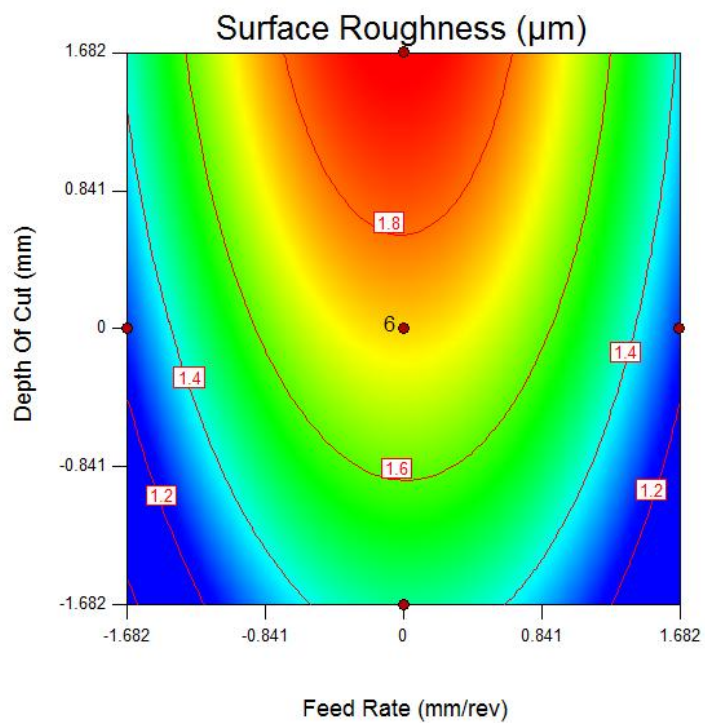
Fig 9: Contour plot of Surface roughness-Feed rate and Depth of cut
