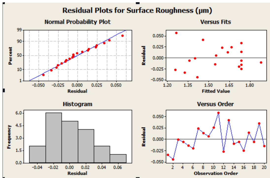
Fig4 : Residual plot for surface roughness (Ra)
