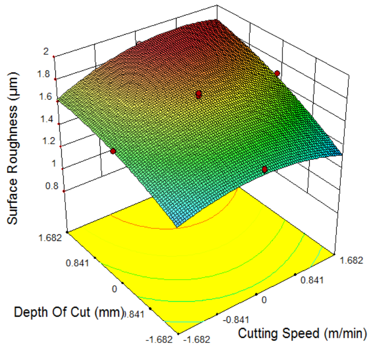
Fig8:Surface plot of Surface roughness-Cutting speed and Depth of cut
