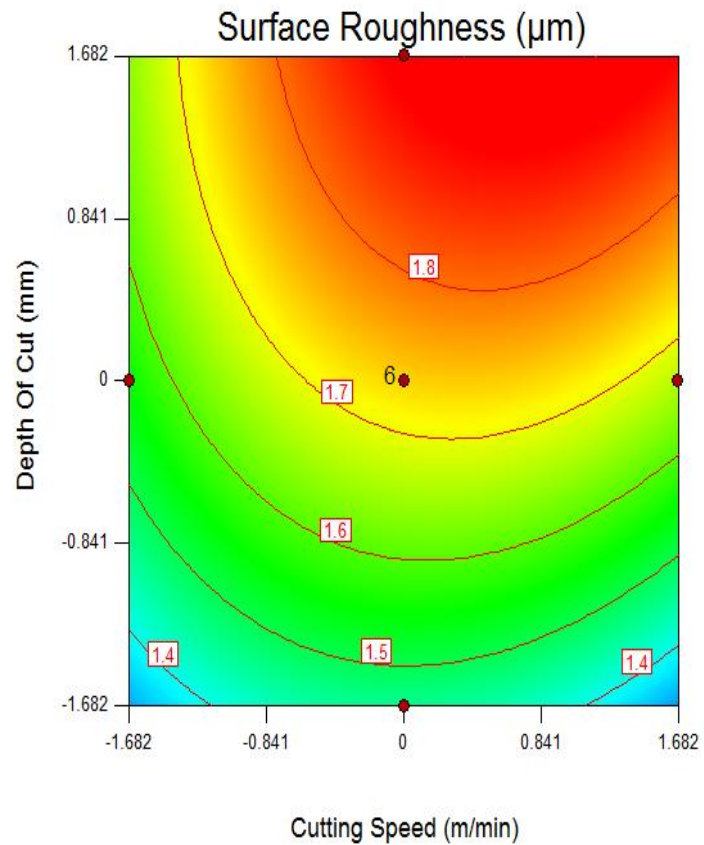
Fig 7: Contour plot of Surface roughness-Cutting speed and Depth of cut.
