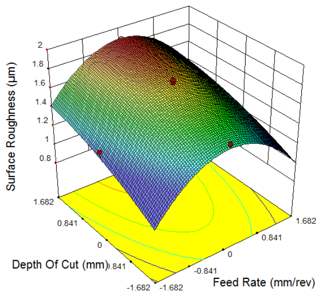
Fig 10: Surface plot of Surface roughness-Feed rate and Depth of cut
