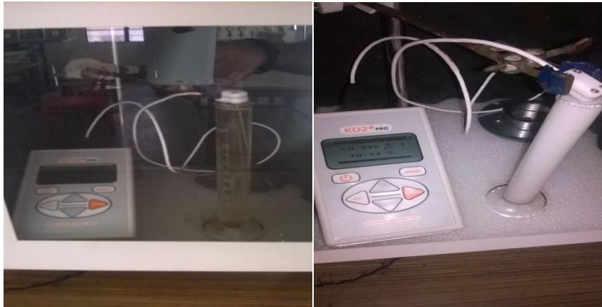
Fig2: Measurement of thermal conductivity with formulated oil and emulsion (20% oil)
