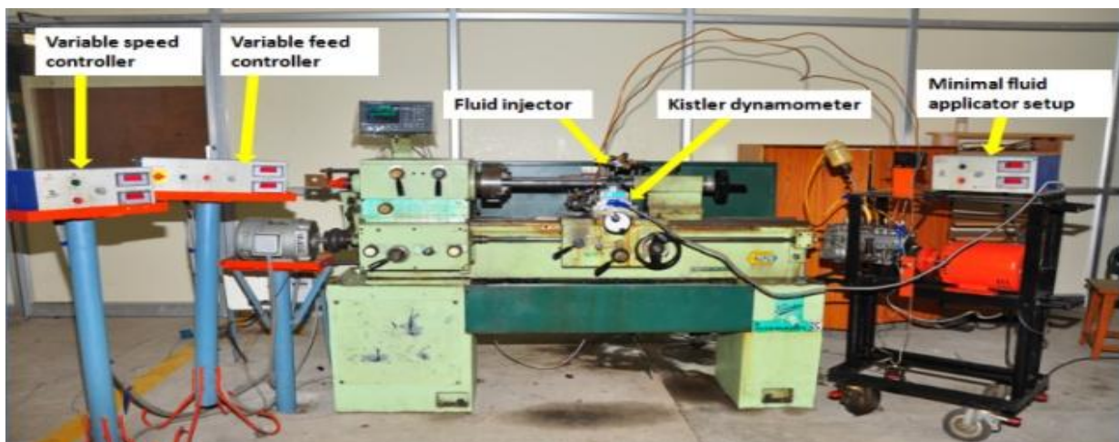
Fig 3 : Lathe With MCFA Setup
