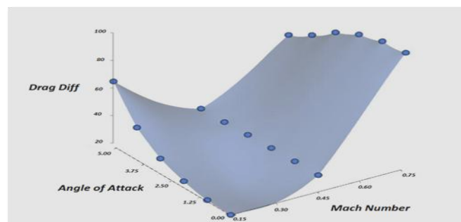
Figure.2: Surrogate model showing the difference in drag values between two different system models.
