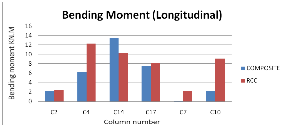
Graph 5 Comparison of bending moment ( Longitudinal Direction )
