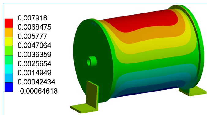
Figure (4) deformation (Strain in E3) in 0.0079 mm.
