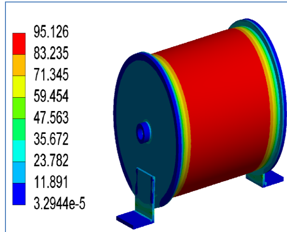
Figure Von mises stress in 95.126 Mpa.
