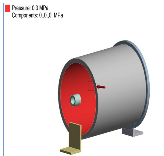
Figure (1) the internal pressure applied on the shell (0.3 Mpa)
