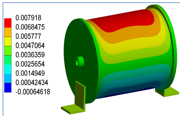
Figure shows deformation (Strain in E1) in 0.0079 mm.
