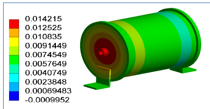
Figure (3) deformation (Strain in E2) in 0.00142 mm.
