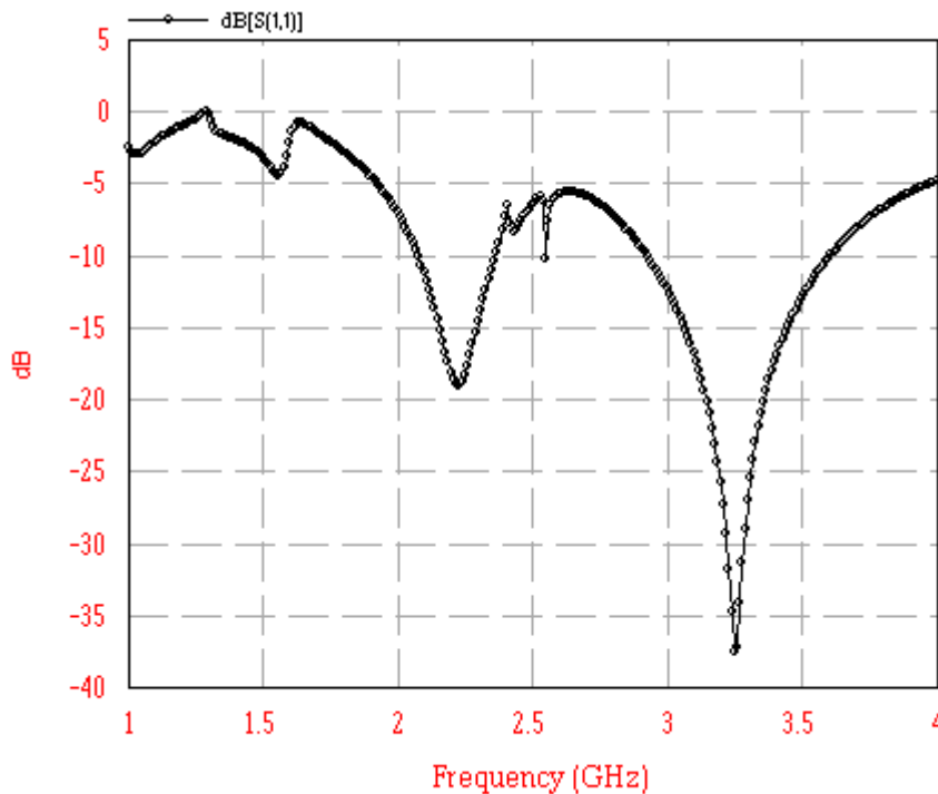
Figure 4. Return loss graph of proposed microstrip antenna
