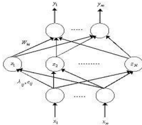
Figure 2. Neural Network approach (Radial Basis Function Network).
