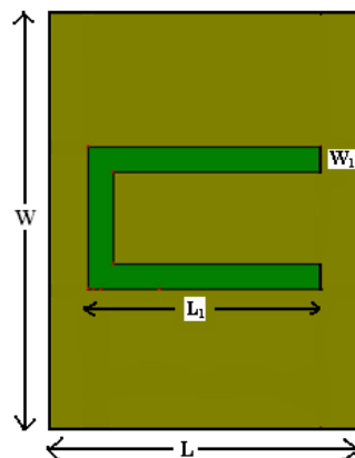
Figure 1. Geometry of proposed microstrip antenna.
