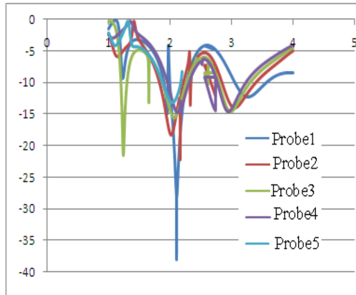
Figure 5. Return loss Vs frequency plot of proposed microstrip antenna for different position of probe feed
