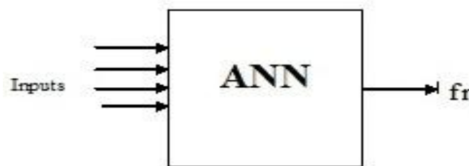
Figure 3. ANN Model.
