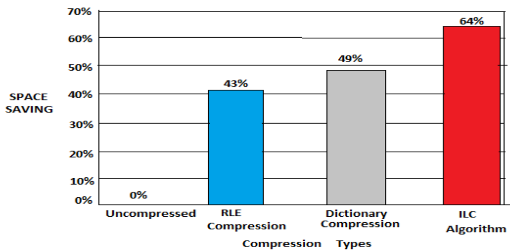
Fig.3. Compression Types vs Space Savings
