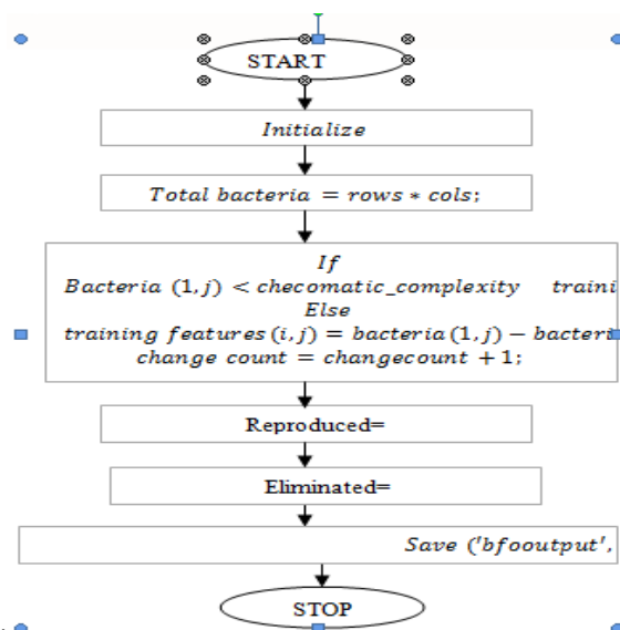
Fig. 1.BFO Flowchart
