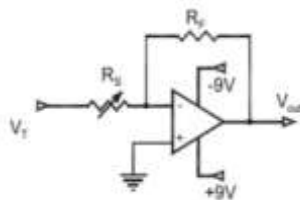
Fig 5 Signal conditioning unit using op amp
