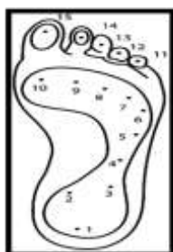
Fig. 2 Foot anatomical areas [12]
