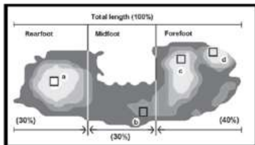
Fig. 1 Pressure regions in human foot [10]
