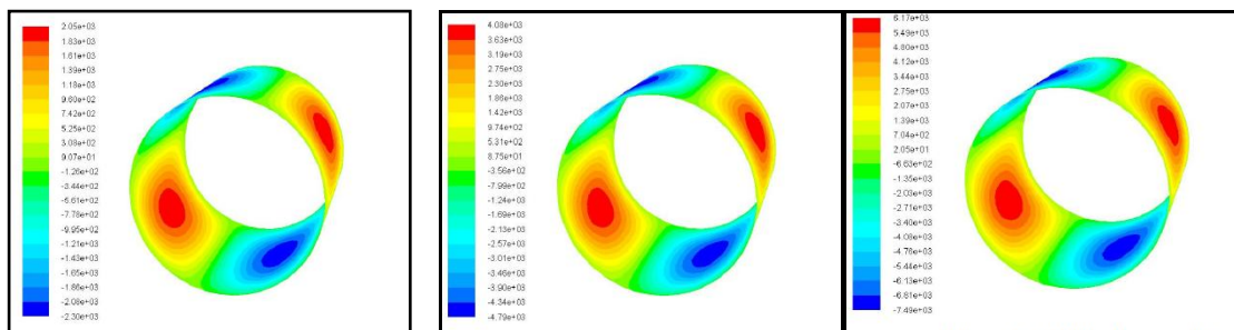
Fig.3: Pressure contour of noncircular hydrodynamic journal bearing with offset factor = 0.8
