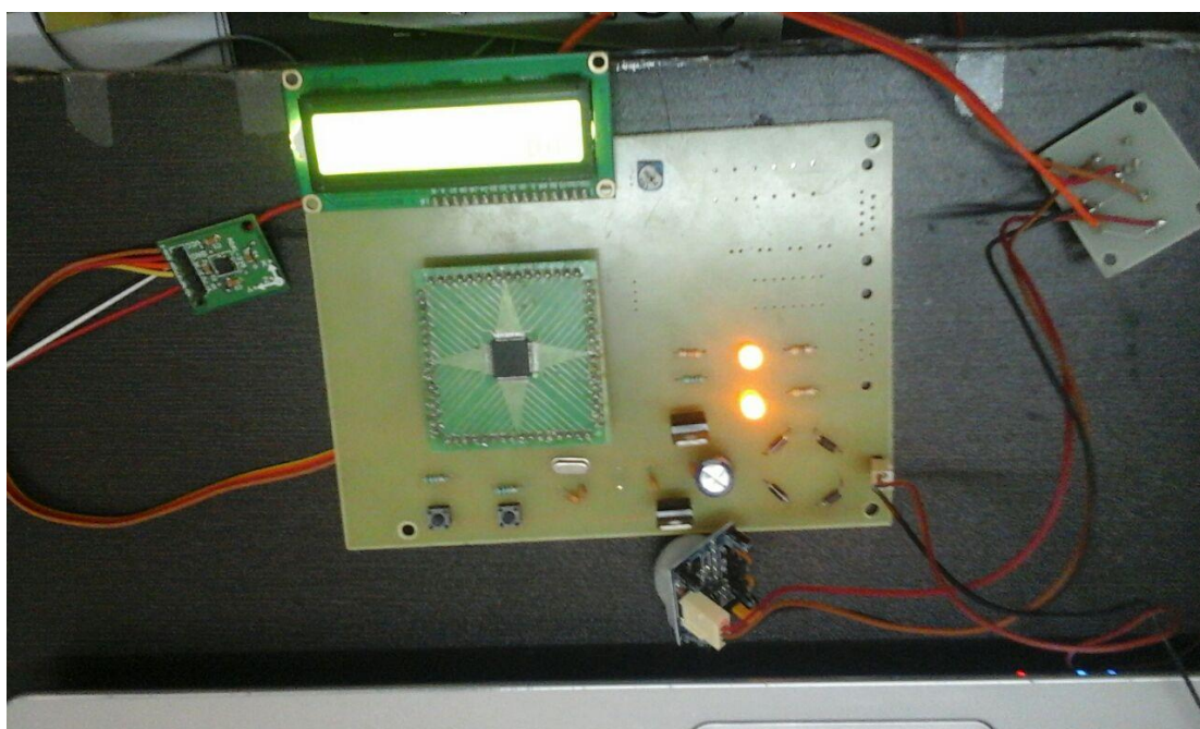
Fig. 5 Hardware implementation for MEMS sensor & PIR sensor
