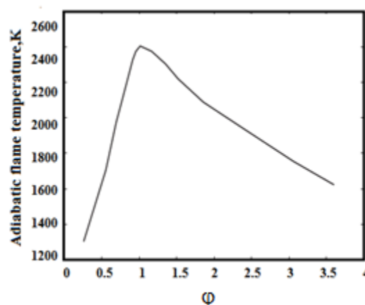
Fig. 1 Adiabatic flame temperature for hydrogen
