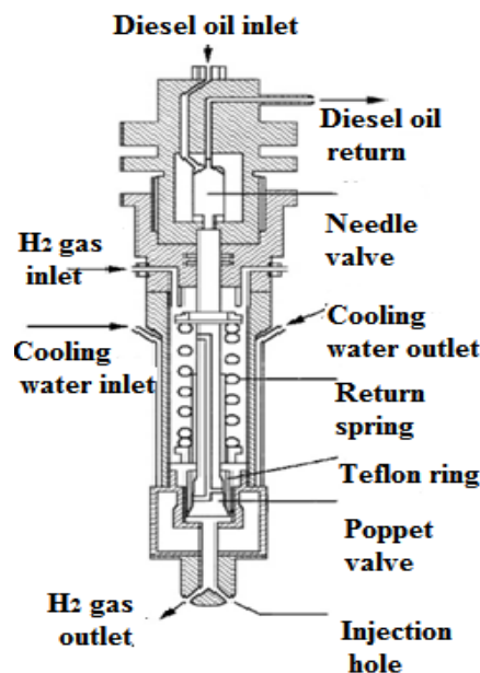
Fig.7. Hydrogen injector [21]
