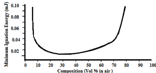
Fig. 3. Minimum ignition energy of hydrogen in air [4]
