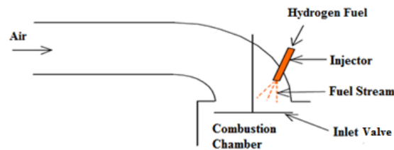
Fig.5. Inlet manifold and inlet port injection [4]
