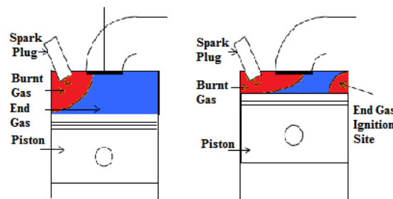
Fig. 9 Knock Out end gas Ignition
