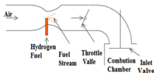
Fig.4. Fuel carburetion method [4]
