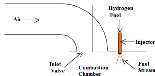
Fig.6. Direct injection system [4]
