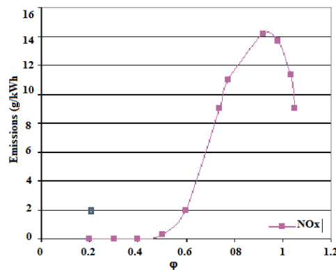
Fig.10 Emissions for a hydrogen eng.
