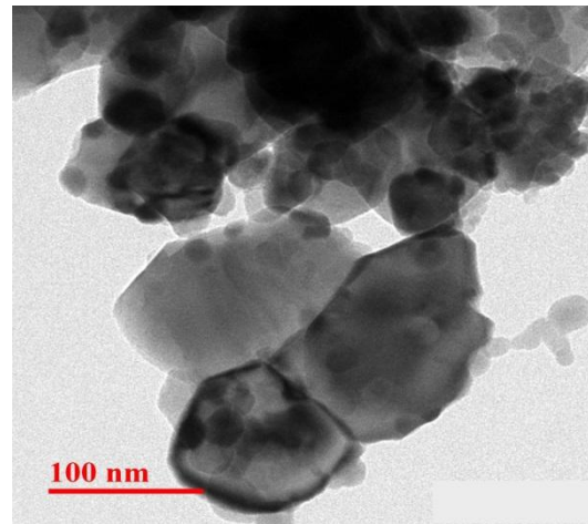
Fig.5 TEM image of 10% Co doped ZnO
