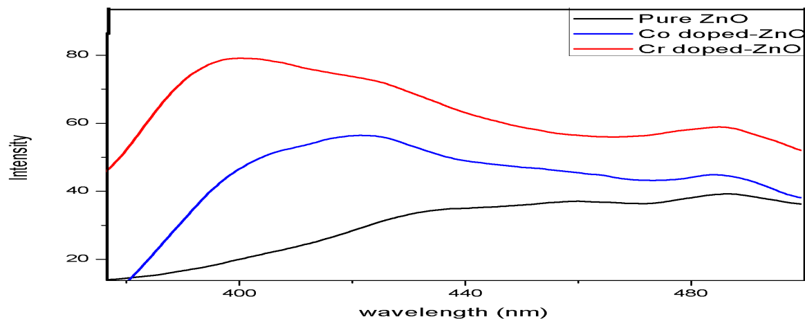
Fig. 7 The PL Emission of Pure and Doped ZnO
