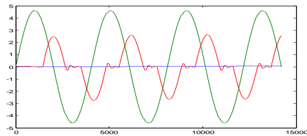
Fig.16. Inductor Current for firing angle 165 deg
