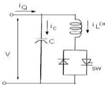
Fig.6. basic FC-TCR type static generator
