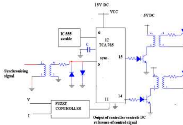
Fig.12. Firing Scheme with TCA 785 IC
