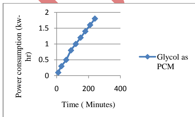
Fig 3.3 Powerconsumtion v/s time for Ethylene glycol.
