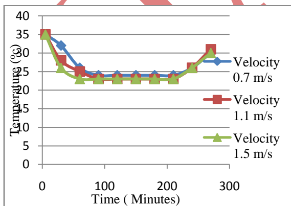
Fig .3.8. Temperature v/s time at different velocities.
