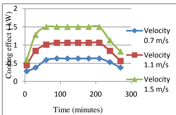
Fig 3.9 Cooling effect v/s time at different velocities
